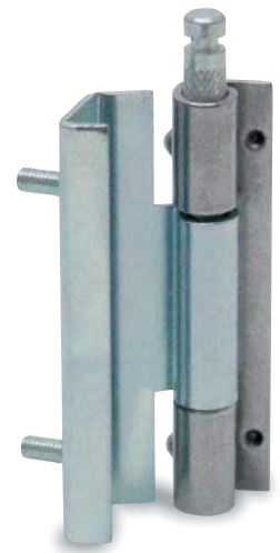
Hinge solution with removable pin for control panel construction
