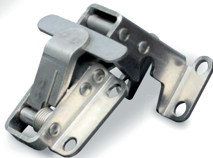
Hood hinge with retaining function for concealed installation
